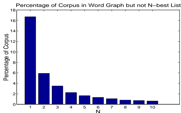
Figure 4: Representation capability
