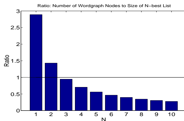
Figure 5: Representation size
