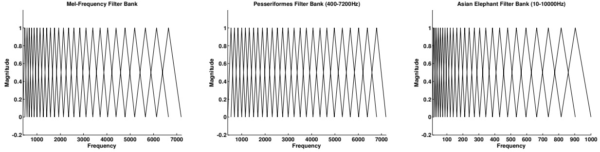
Figure 1: Filter Bank Comparison between Mel-Scale and Greenwood Scale for Passeriformes and Asian Elephants
