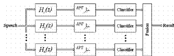
Fig. 3. System diagram of the proposed phoneme classification system.
